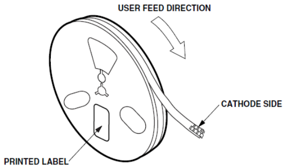
Figure 12: Reel Orientation
