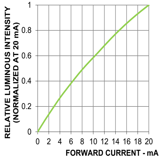
Figure 3: Luminous Intensity vs. Forward Current
