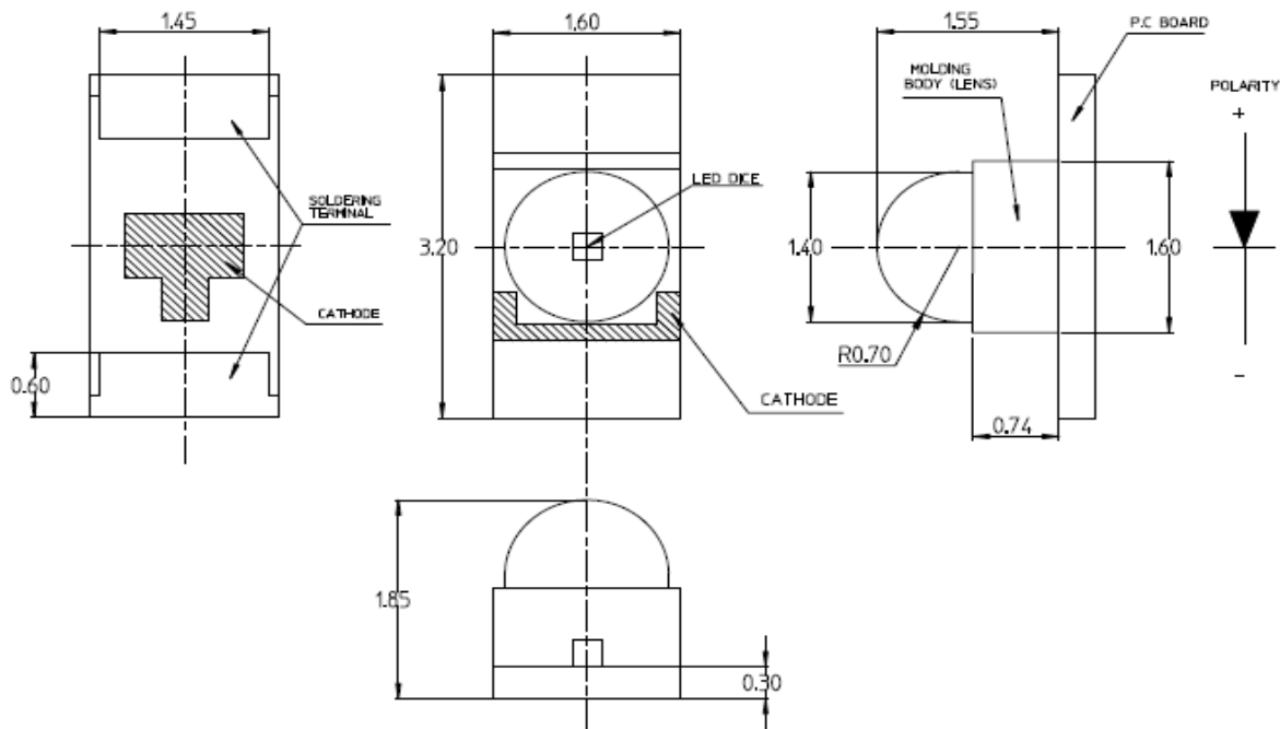
Figure 1: Package Dimensions
