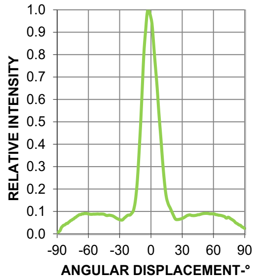
Figure 5: Radiation Pattern
