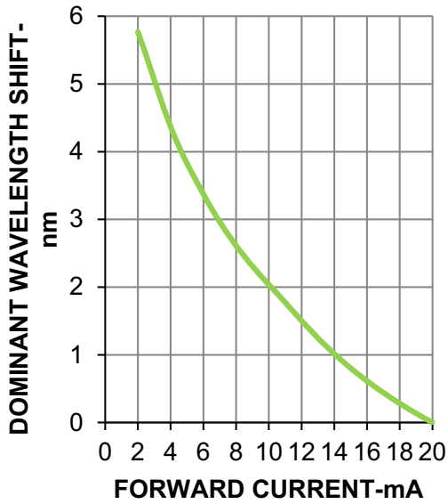
Figure 6: Wavelength Shift vs. Forward Current
