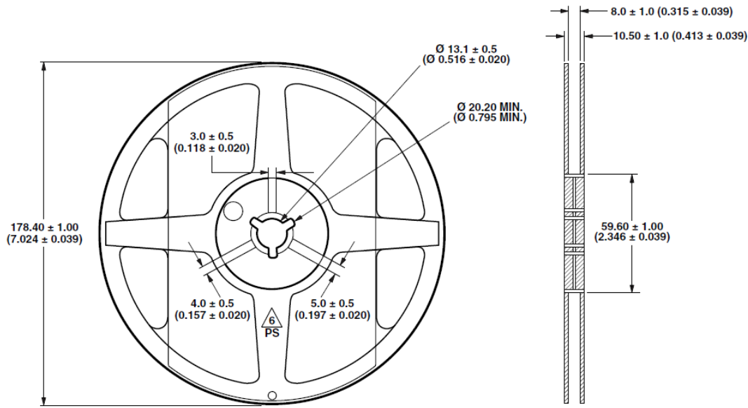
Figure 13: Reel Dimensions
