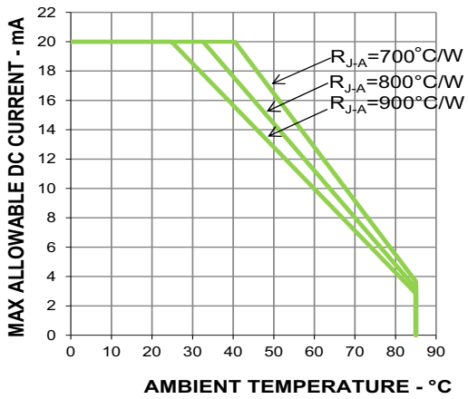
Figure 10: Derating Curve
