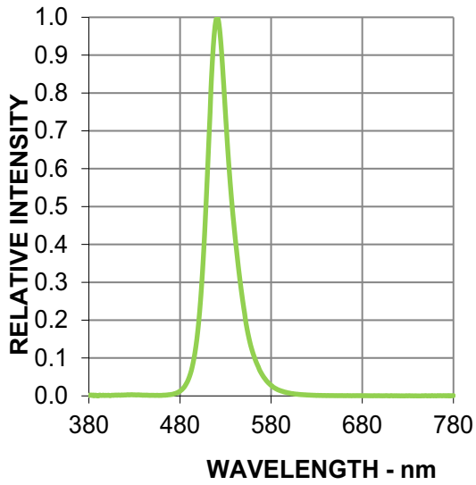
Figure 2: Spectrum
