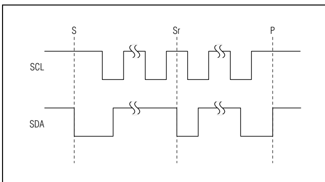
Figure 4. START, STOP, and REPEATED START Conditions
