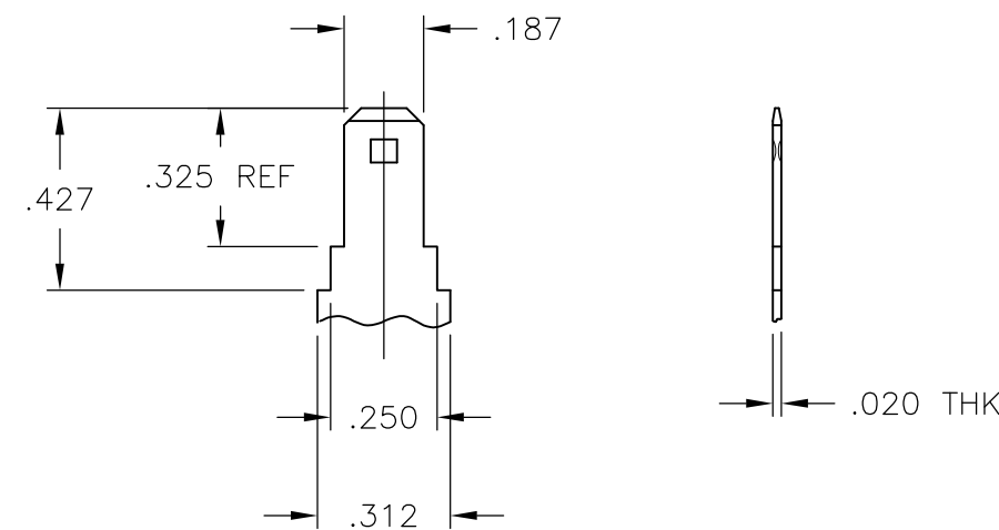
DETAIL OF MALE TAB SCALE 2:1
