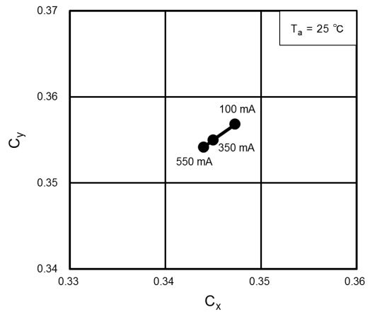
Fig. 8.4 Chromaticity - I_F
